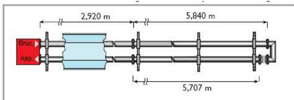
PANRAD FRB – dl.9m, z trubek dl. 6+3m
